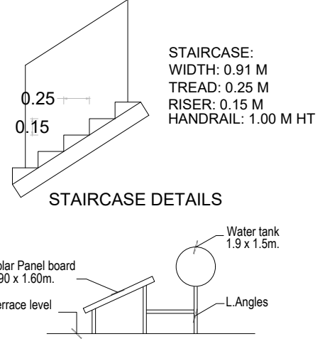
SOLAR WATER HEATING SYSTEM (NOT TO SCALE)
