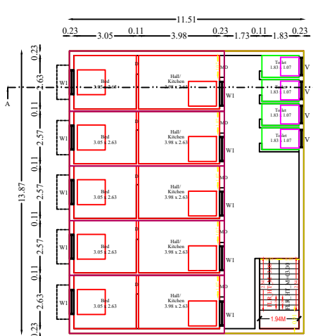
Pro. Second Floor Plan
