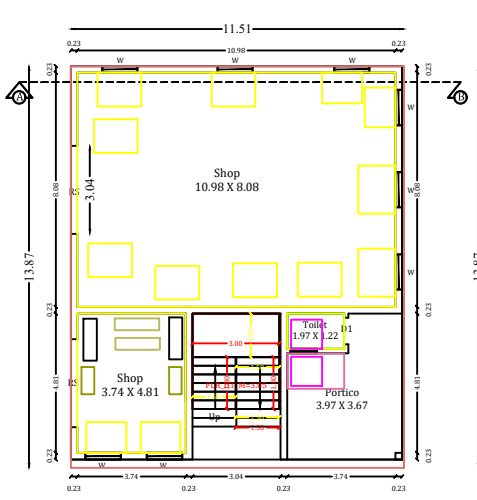
Exg.Ground Floor Plan
