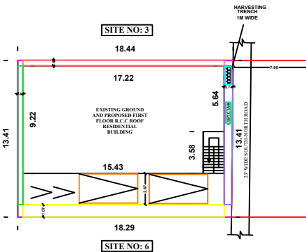
SITE PLAN
