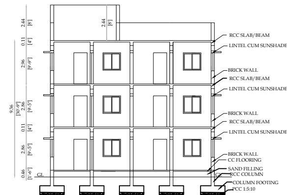
SECTION "A-B"
