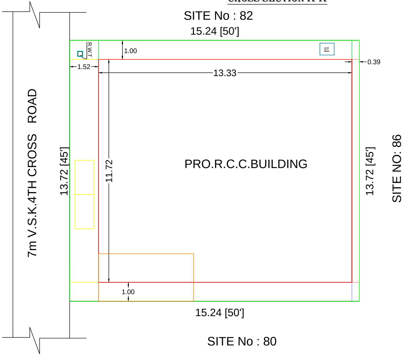
SITE PLAN
