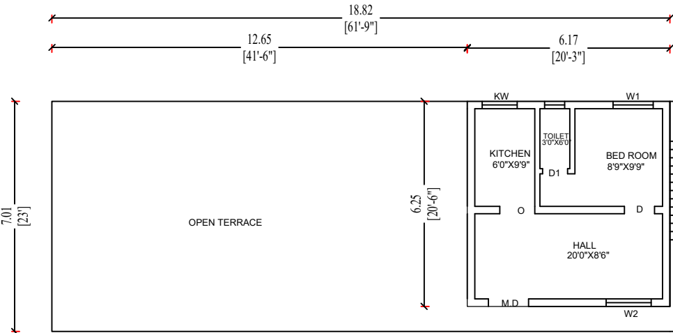
PROPOSED FIRST FLOOR
