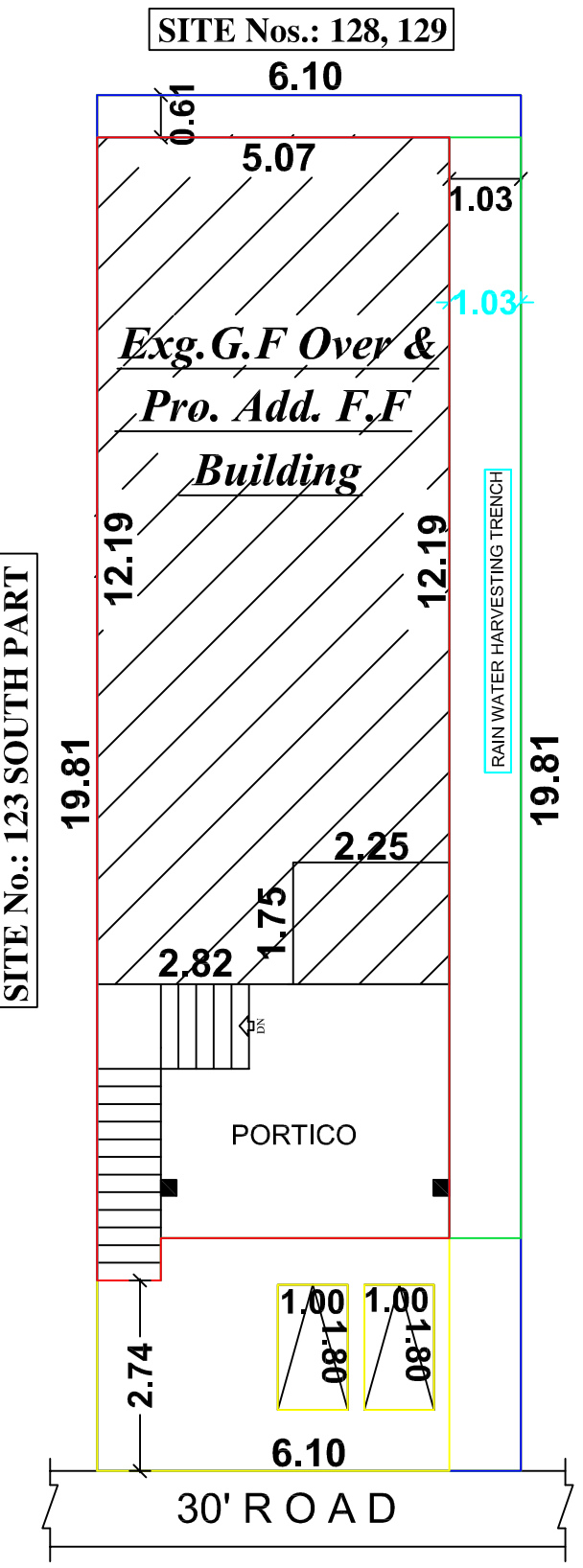
SITE PLAN
