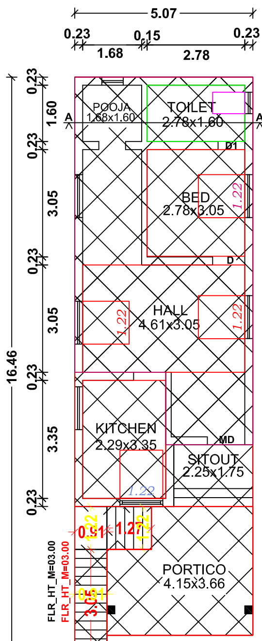
D FLOOR PLAN
