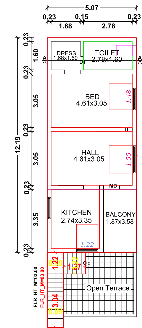
PRO. ADD. FIRST FLOOR PLAN
