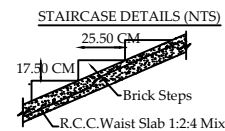
STAIRCASE DETAILS (NTS)
