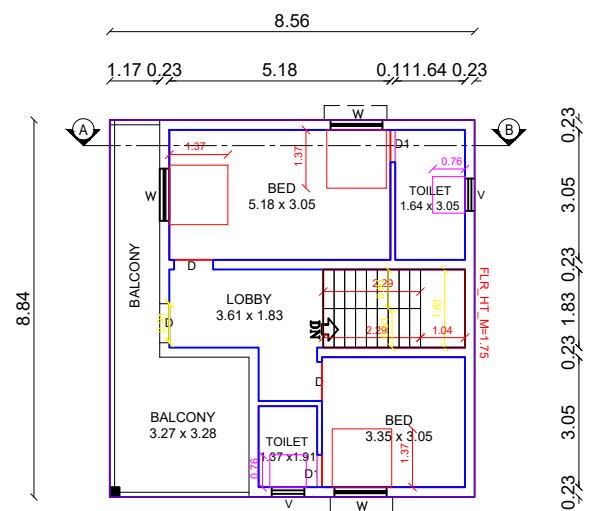
PRO.ADDL.FIRST FLOOR PLAN
