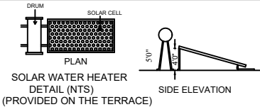
SOLAR WATER HEATER DETAIL (NTS) (PROVIDED ON THE TERRACE)
