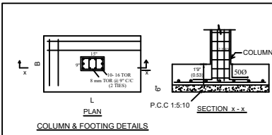
COLUMN & FOOTING DETAILS
