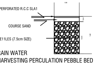
RAIN WATER HARVESTING PERCOLATION PEBBLE BED
