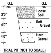
TRIAL PIT (NOT TO SCALE)
