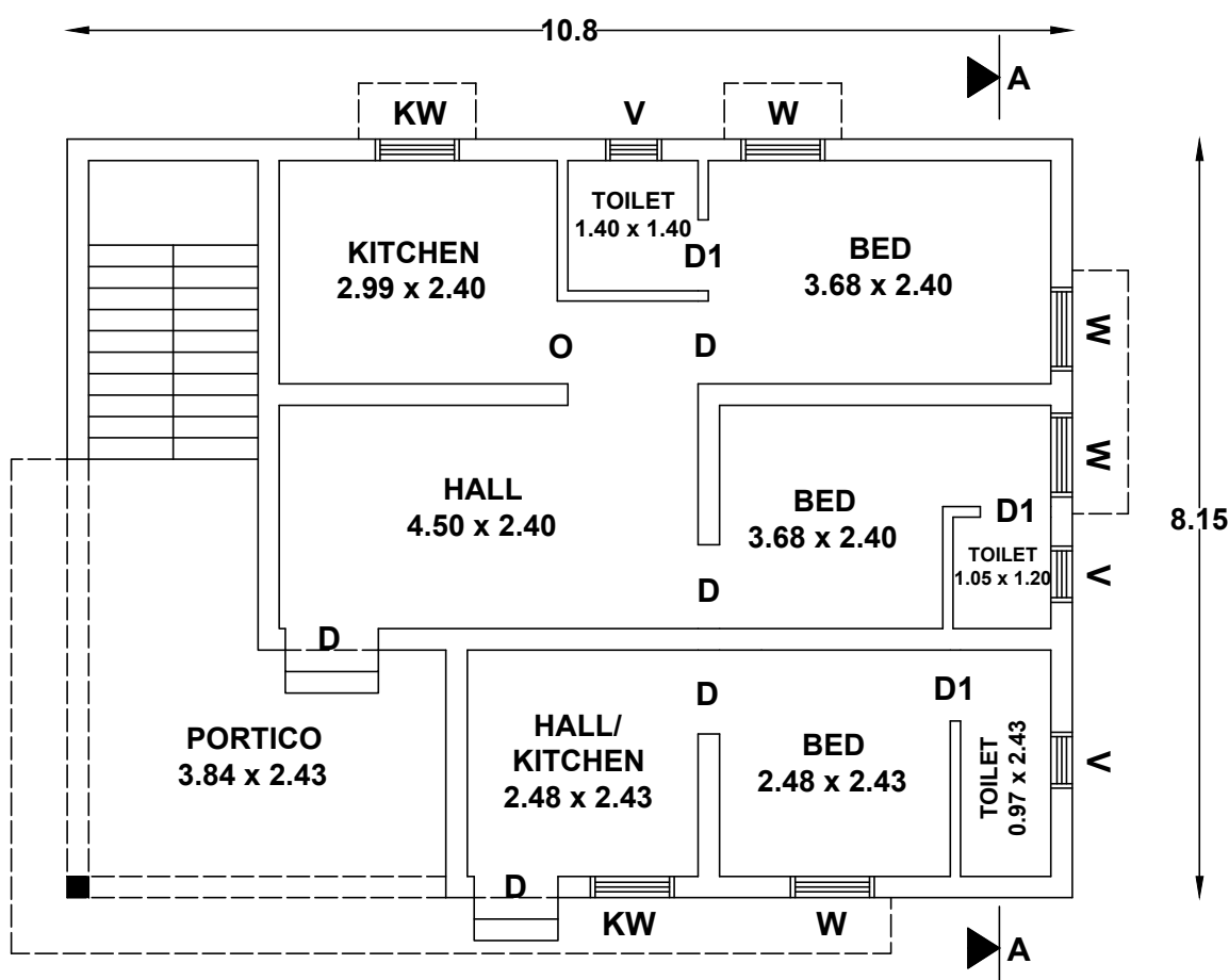
GROUND FLOOR PLAN SCALE - 1' 0" = 8' 0"
