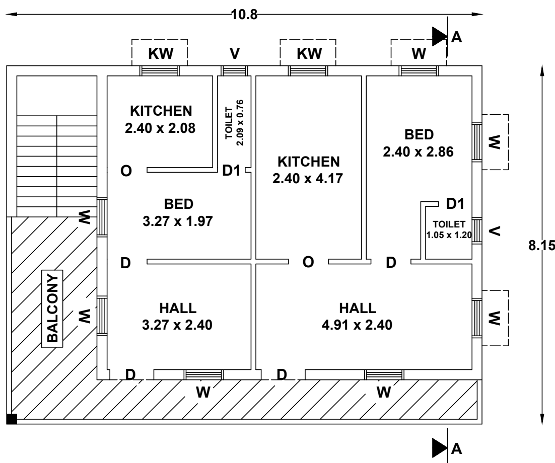
FIRST FLOOR PLAN SCALE - 1' 0" = 8' 0"
