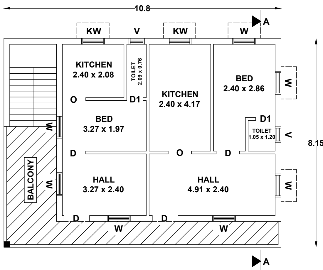
SECOND FLOOR PLAN SCALE - 1' 0" = 8' 0"
