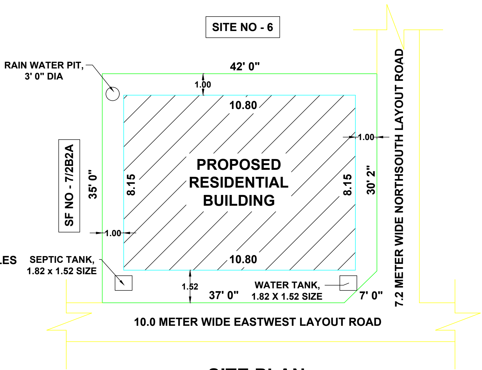
SITE PLAN SCALE - 1' 0" = 10' 0"
