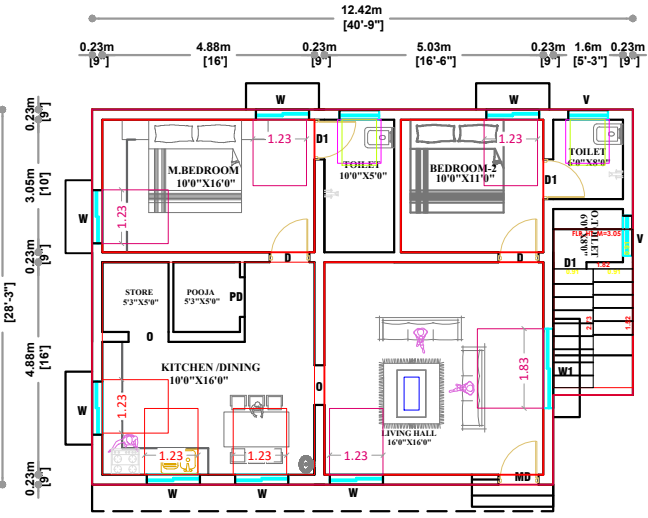
PROPOSED GROUND FLOOR BUILDING
