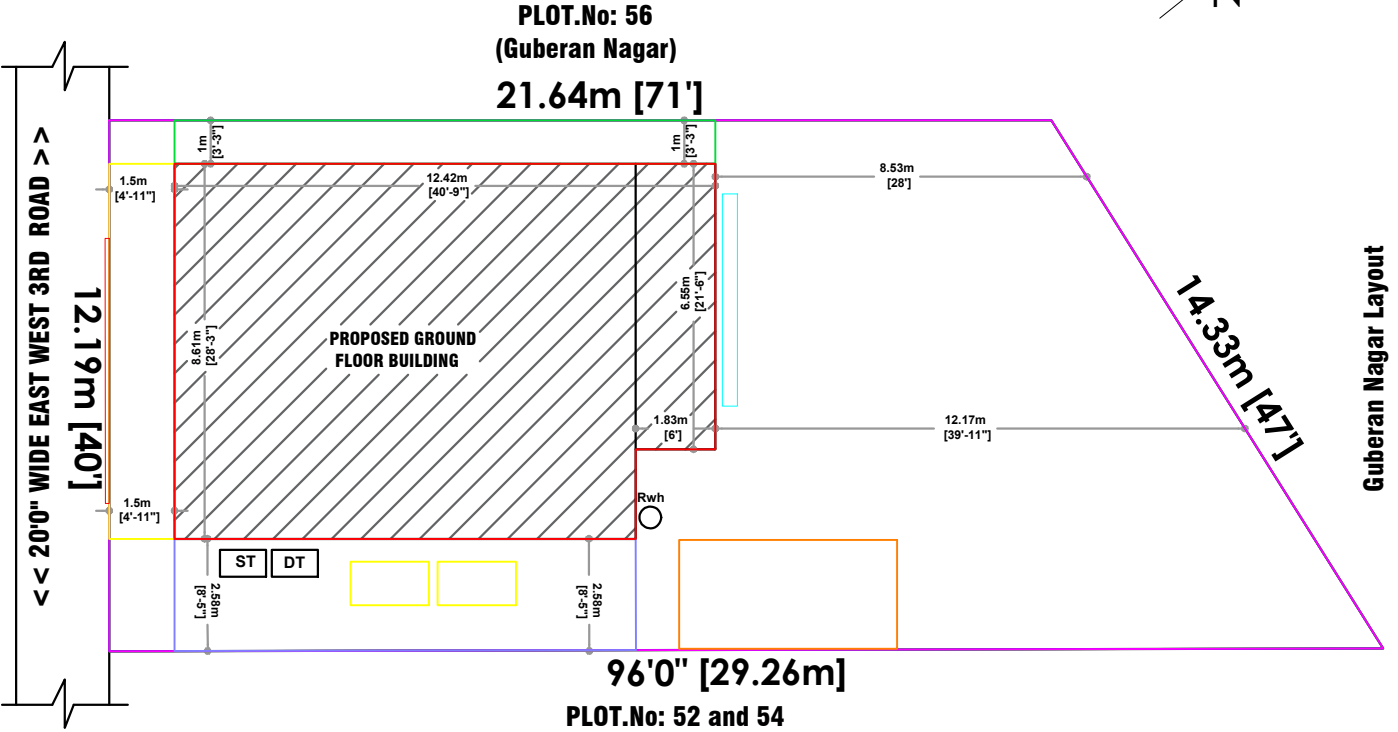
SITE PLAN
