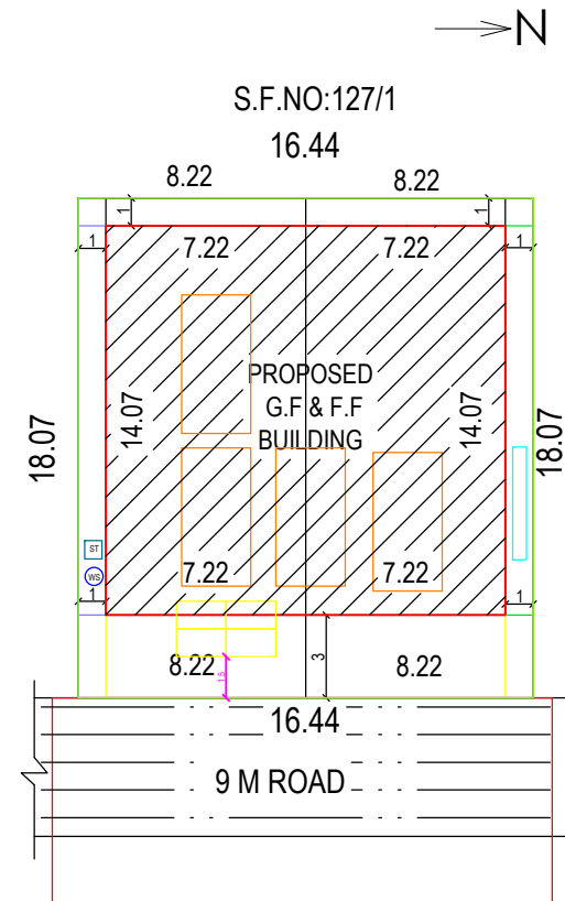
SITE PLAN
