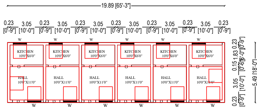
PROPOSED PLAN
