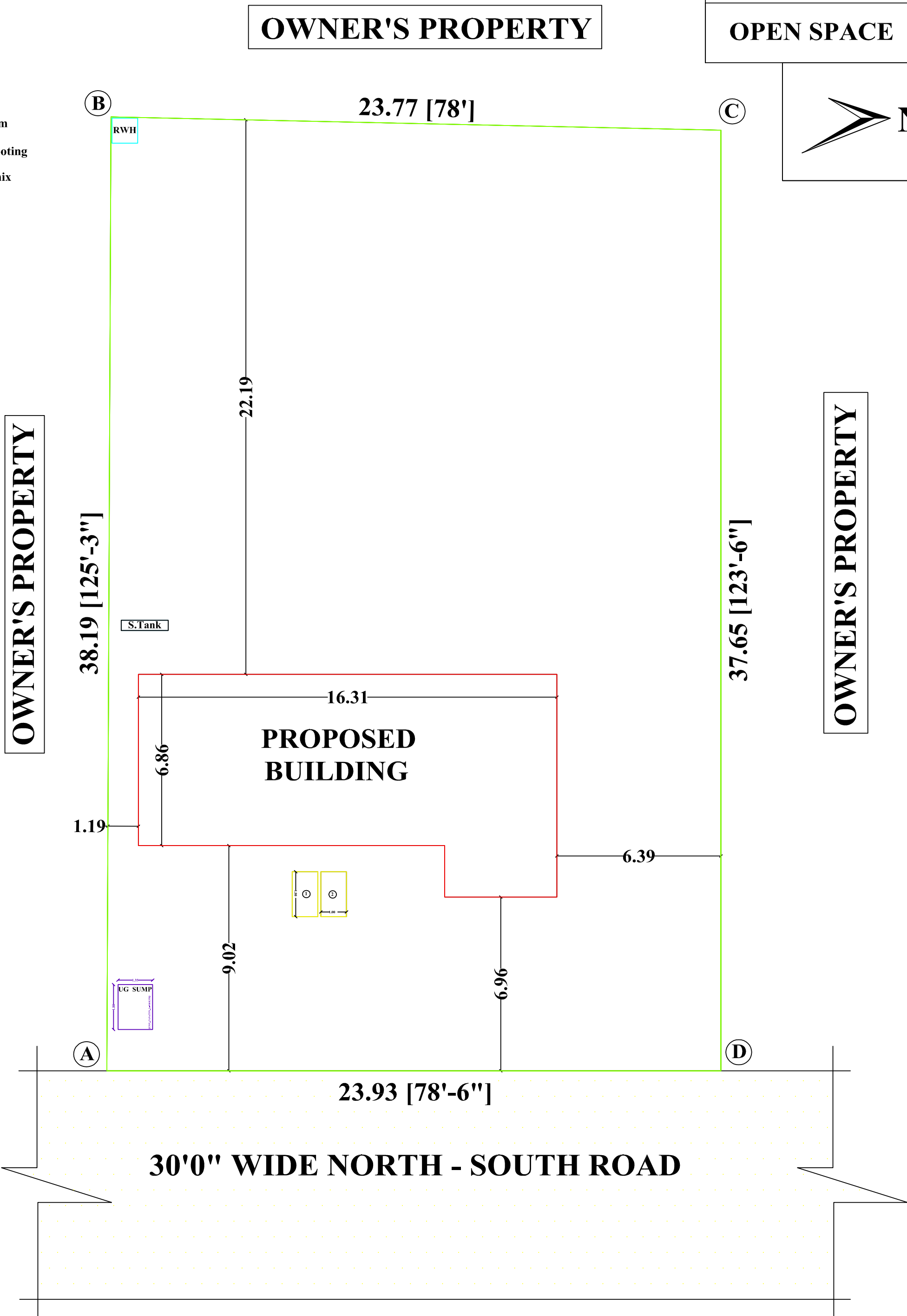
SITE PLAN
