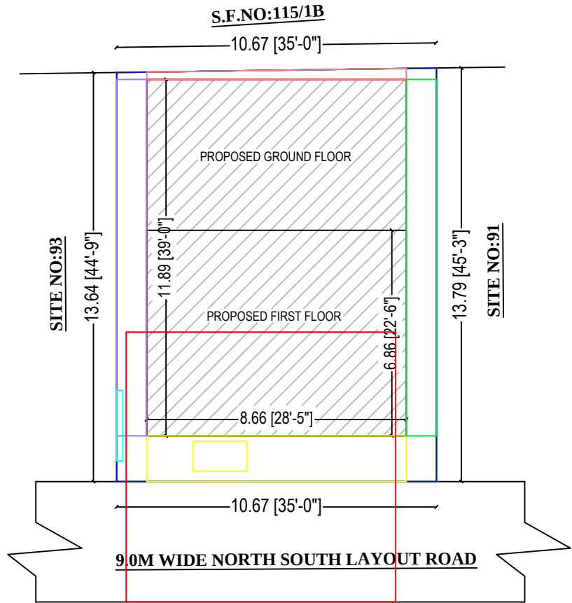
SITE PLAN
