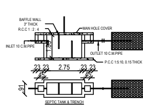
SEPTIC TANK & TRENCH
