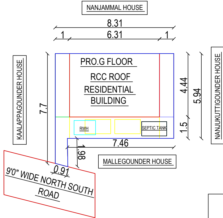
SITE PLAN
