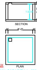
SECTION PLAN RW_H_CAPACITY_L=5000LTRS
