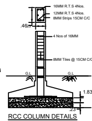
RCC COLUMN DETAILS
