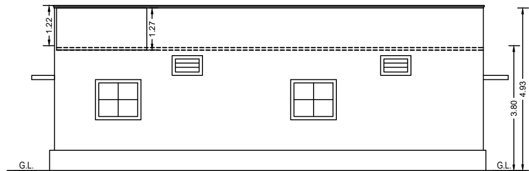
Elevation - (East - Side)
