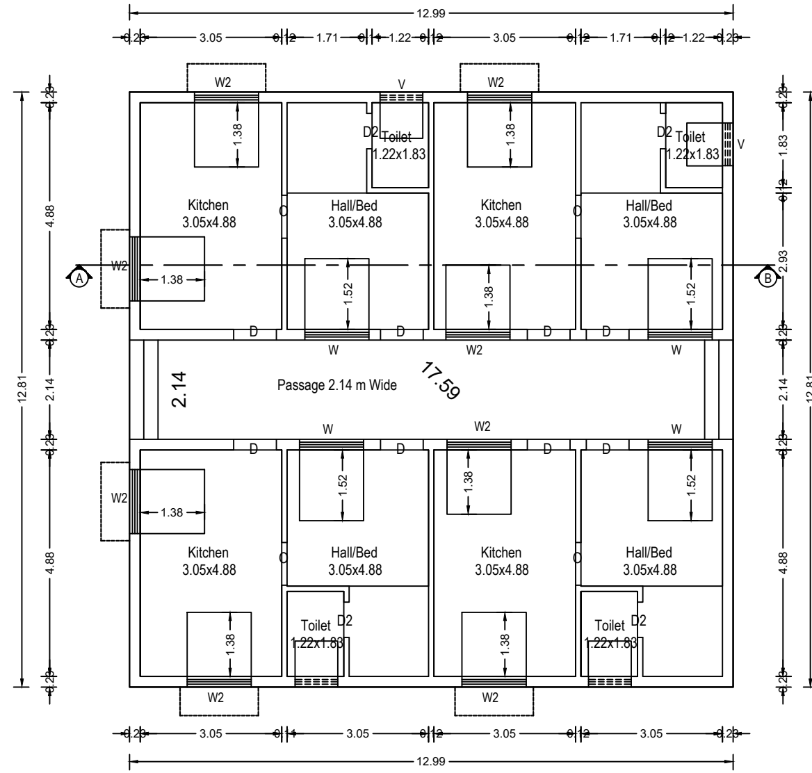
Plan Scale 1:100 Ground floor
