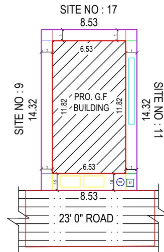
SITE PLAN
