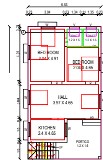
PROPOSED GROUND FLOOR BUILDING
