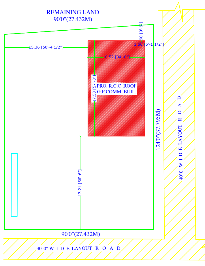
SITE PLAN
