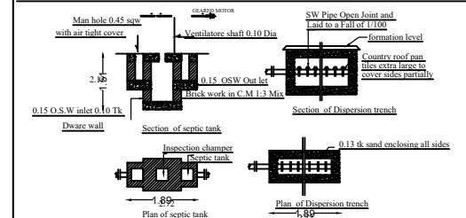
TAILED DRAWING FOR SEPTIC TANK WITH DISPERSION TRENCH 225 GALONS CAPACITY OF 1000 LITRES
