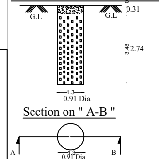
TAILED DRAWING FOR SEPTIC TANK WITH DISPERSION TRENCH 225 GALONS CAPACITY OF 1000 LITRES
