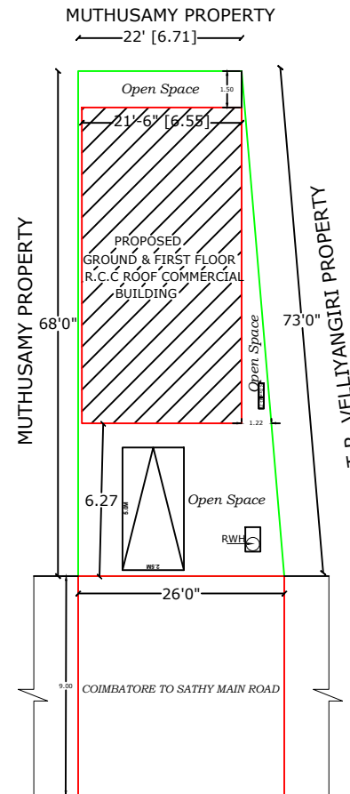
SITE PLAN
