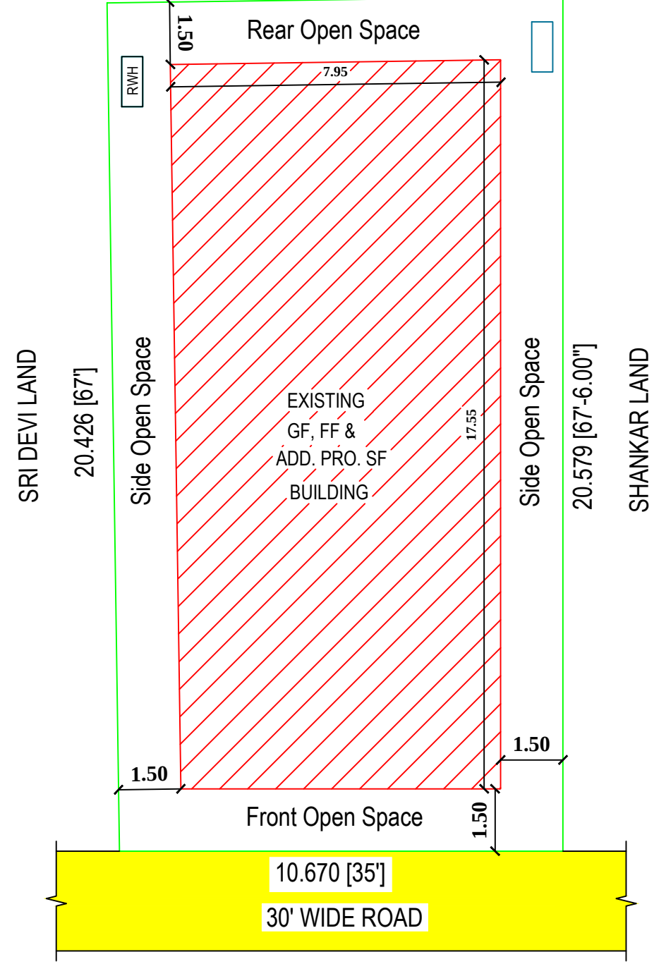
SITE PLAN
