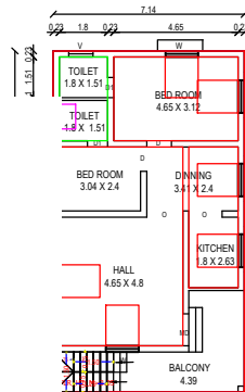
PROPOSED ADDITIONAL 1ST FLOOR BUILDING
