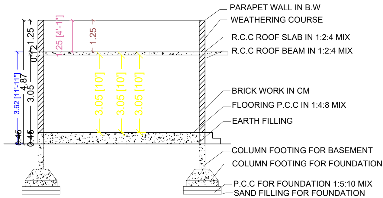
SECTION ON-AA
