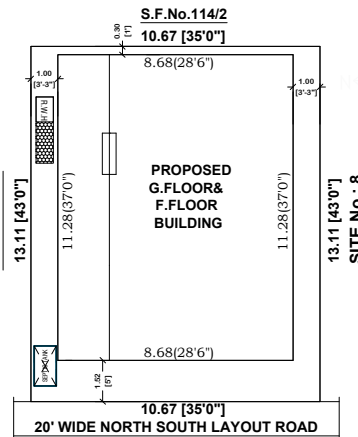
SITE PLAN
