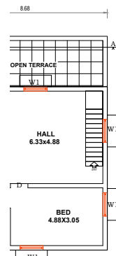
T FLOOR PLAN
