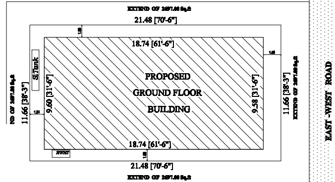
SITE PLAN
