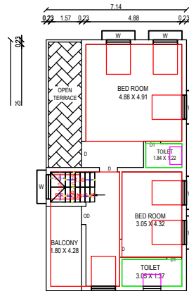
PROPOSED ADDITIONAL FIRST FLOOR PLAN
