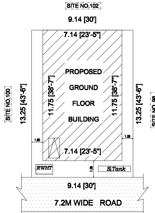
SITE PLAN
