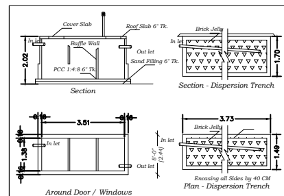
DETAILED PLAN OF RAINWATER PERCOLATION BED
