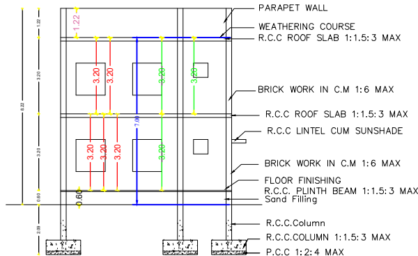
SECTION
