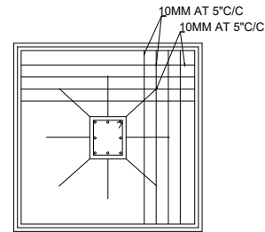
FOOTING DETAIL SCALE: NTS
