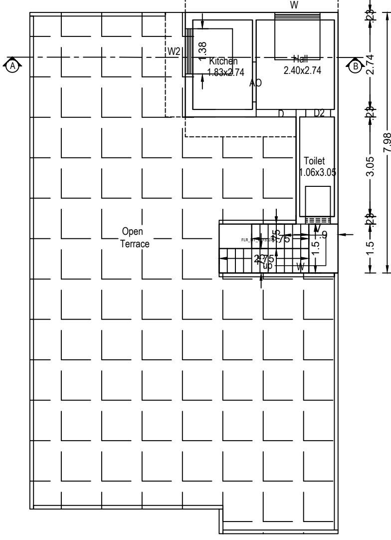
Plan Scale 1:100 First floor
