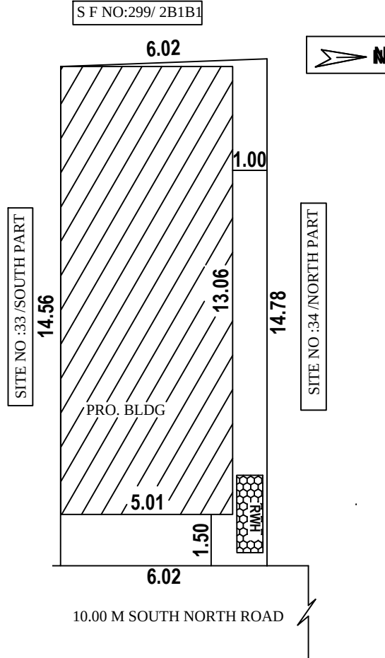
SITE PLAN
