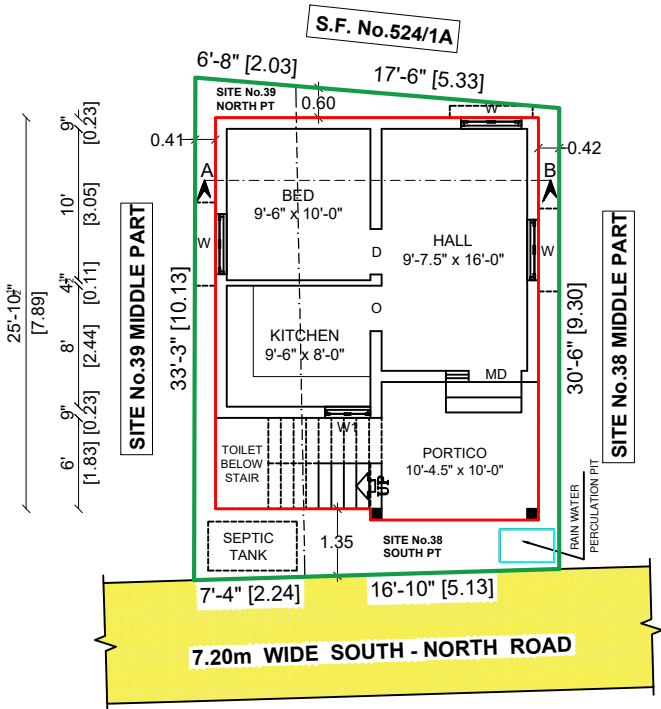
SITE CUM GROUND FLOOR PLAN
