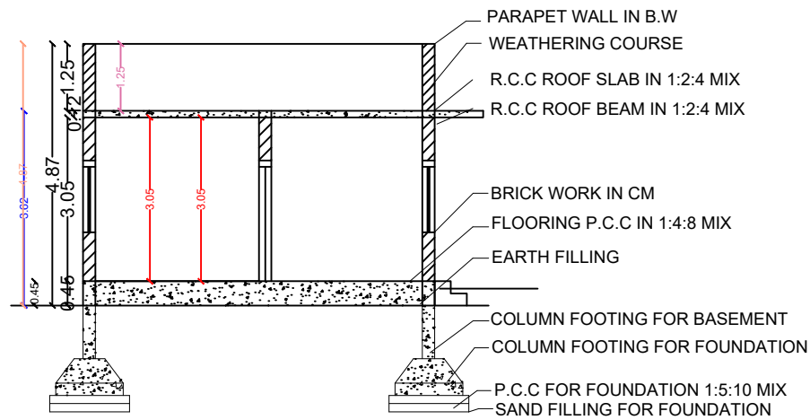
SECTION ON-AA
