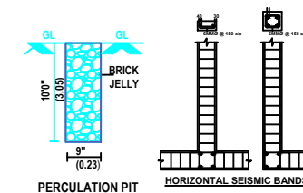
PERCOLATION PIT
