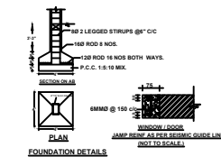
FOUNDATION DETAILS
