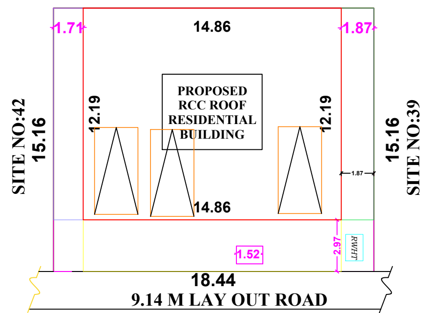
SITE PLAN
