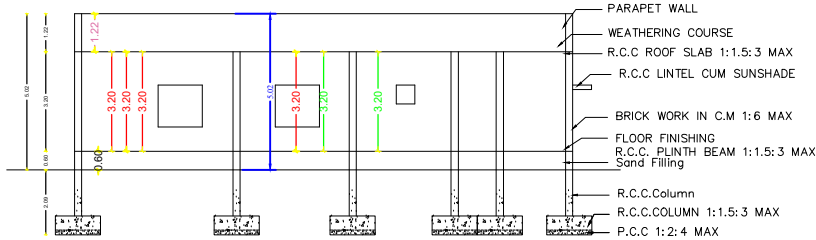
SECTION
