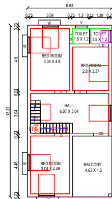
PROPOSED FIRST FLOOR BUILDING
