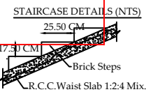
STAIRCASE DETAILS (NTS)
