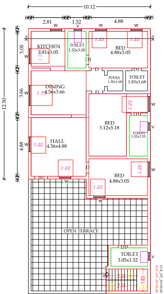
PRO. ADD. FIRST FLOOR
