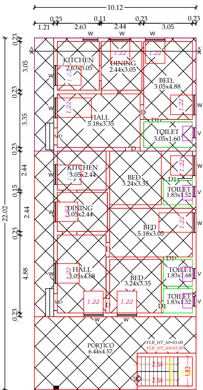
EXI. GROUND FLOOR
