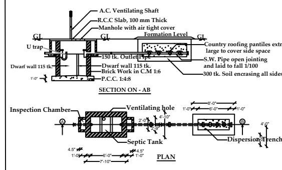
SEPTIC TANK WITH DISPERSION TRENCH (250 Gls.)
