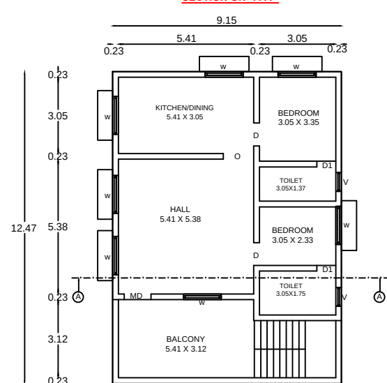
ADD.PROPOSED FIRST FLOOR
