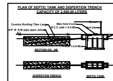
PLAN OF SEPTIC TANK AND DISPOSAL TRENCH
