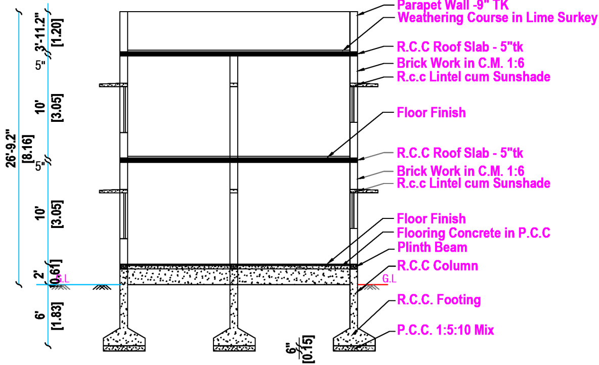
SECTION "AB"
