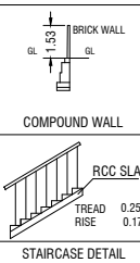
STAIRCASE DETAIL
