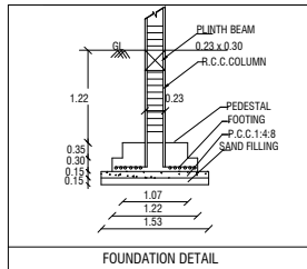
FOUNDATION DETAIL
