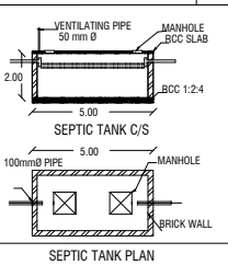
SEPTIC TANK PLAN
