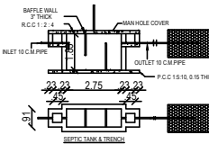
SEPTIC TANK & DRAINAGE
