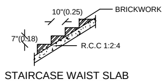
STAIRCASE WAIST SLAB
