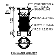
RAIN WATER HARVEST
