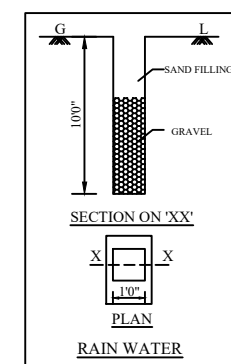
RAINWATER HARVESTING
