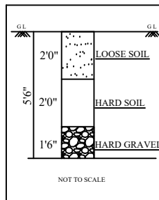
TRIAL PIT
