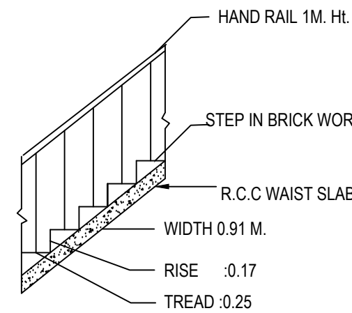
STAIR DETAIL
