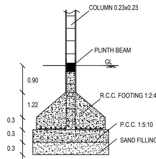
COLUMN DETAILS
