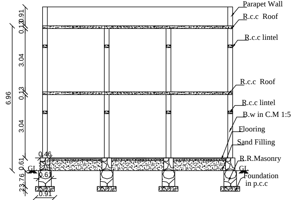
SECTION A&B
