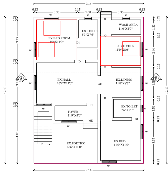
ADDITIONAL EXISTING GROUND FLOOR PLAN
